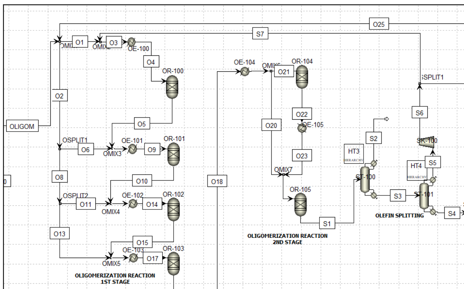
Figure 35- Oligomerization of Ethylene to Oligomers Simulation PFD
