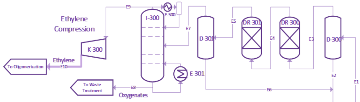
Figure 27- Ethylene Purification Section
