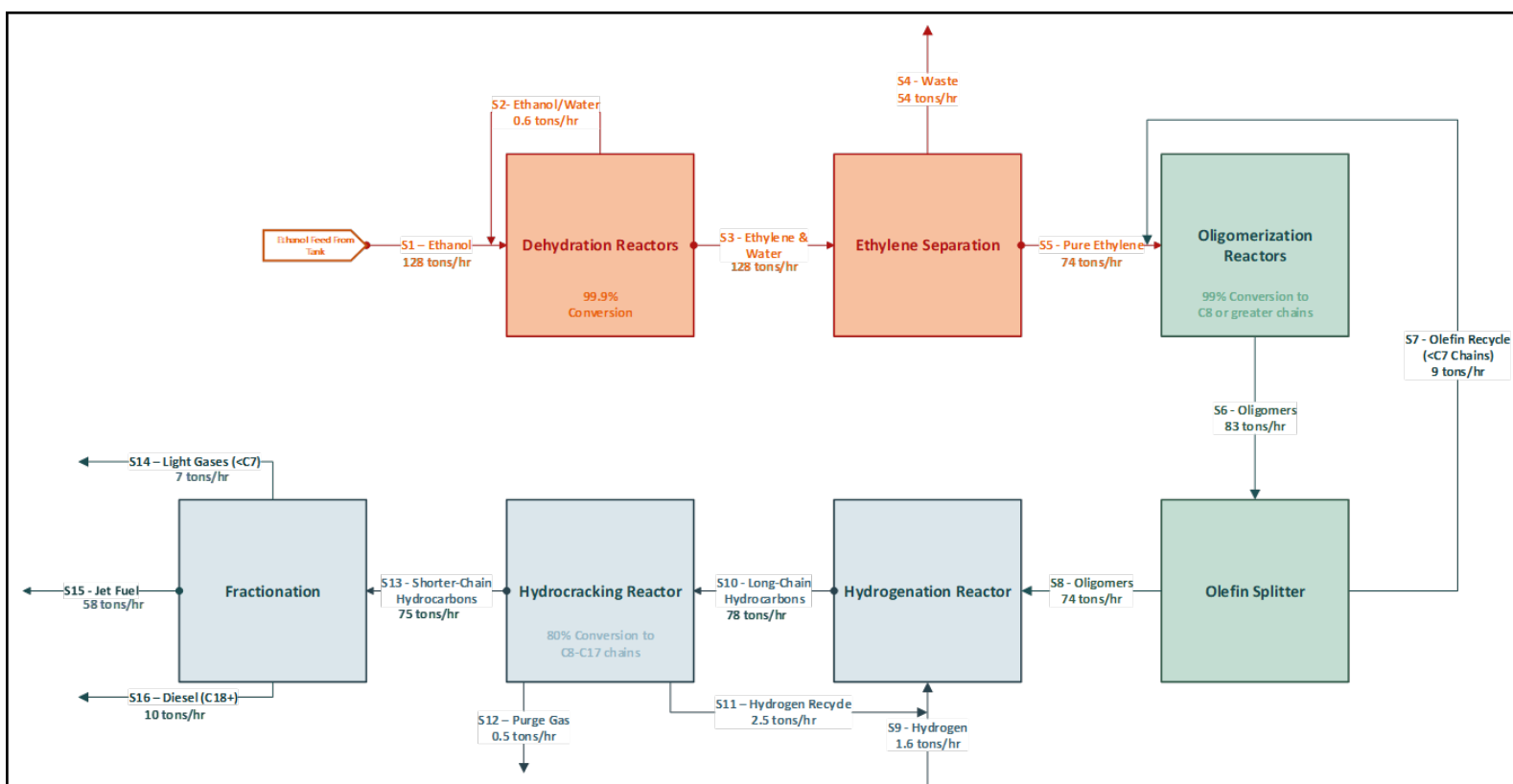
Figure 23- Ethanol to Jet Fuel BFD
