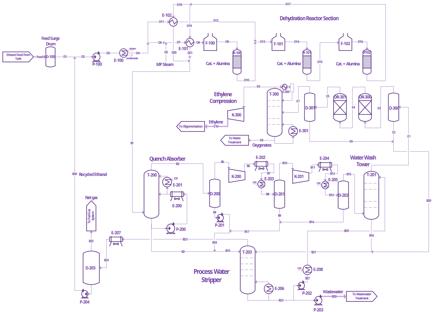
Figure 24- Dehydration of Ethanol to Ethylene PFD
