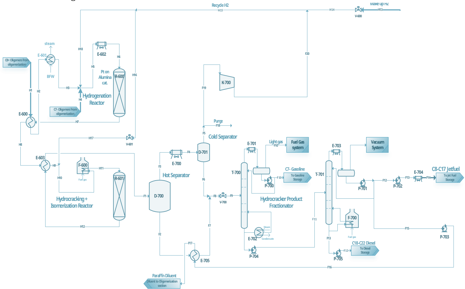
Figure 31- Hydroprocessing Oligomers to Jet Fuel PFD
