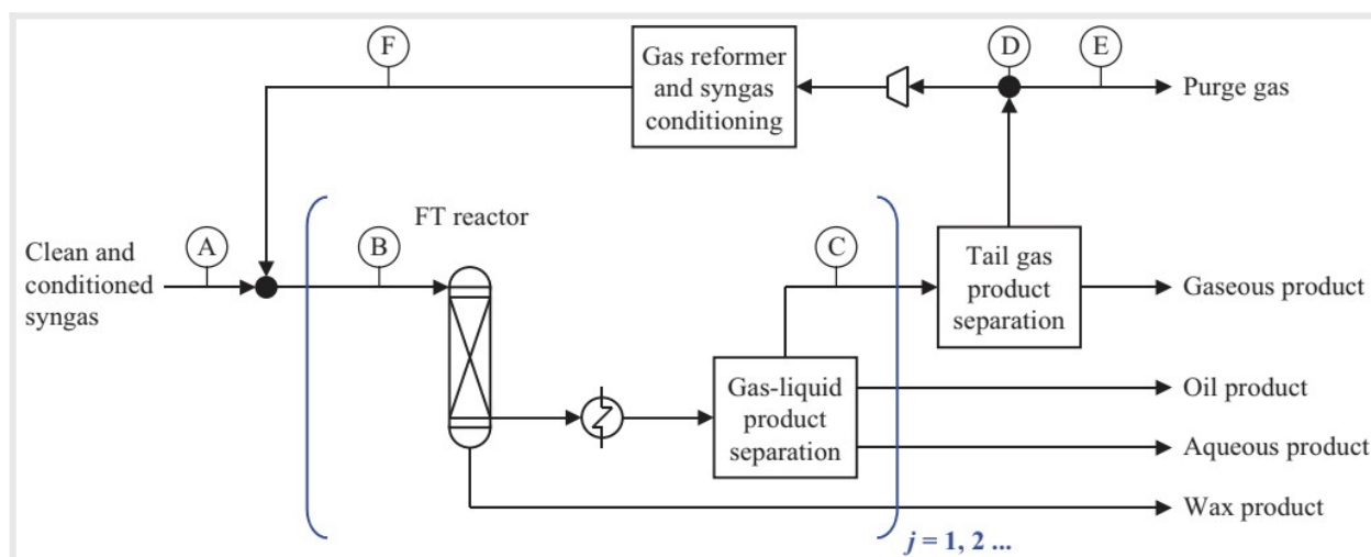
Figure 12: gFT block flow diagram
