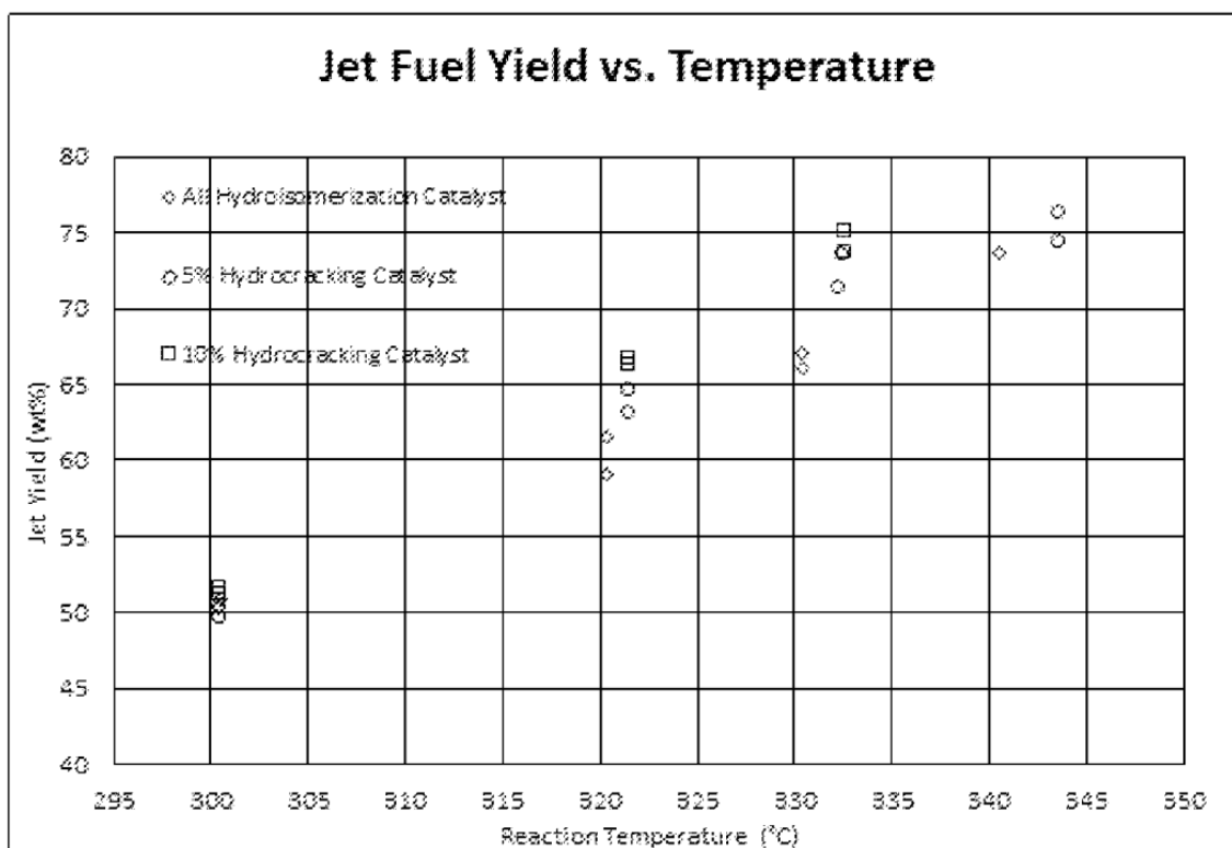
Figure 17- Jet Fuel Yield vs. Temperature [21]
