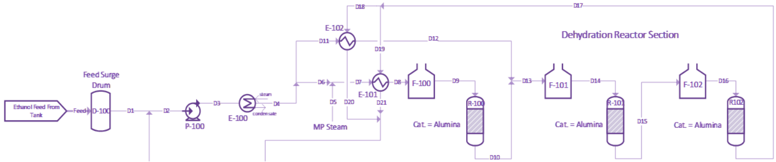
Figure 25- Dehydration Reactor Section
