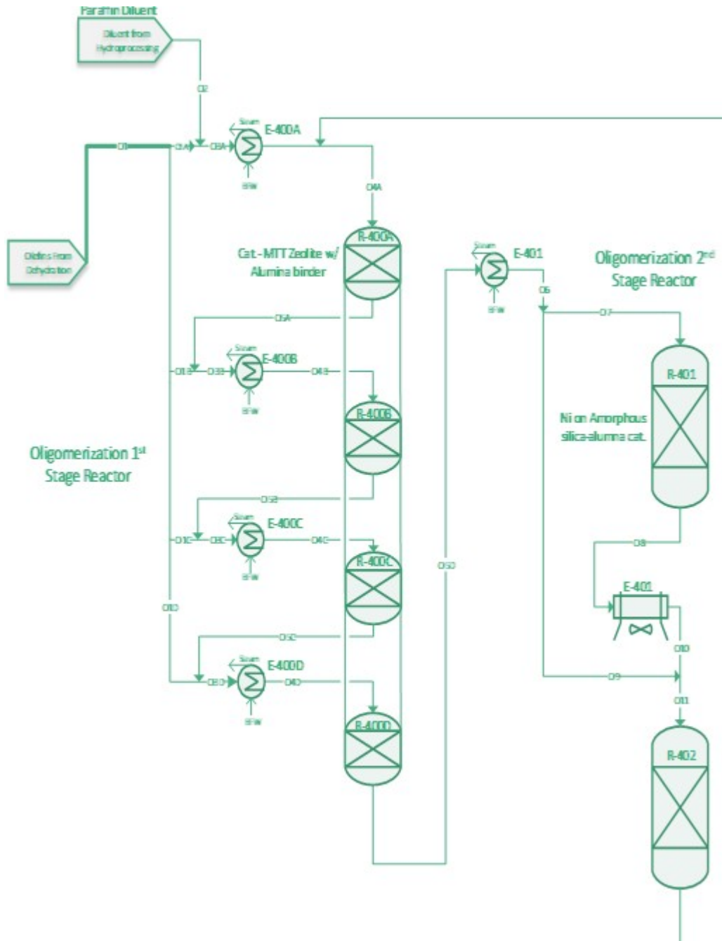
Figure 29- Oligomerization Reactor Section
