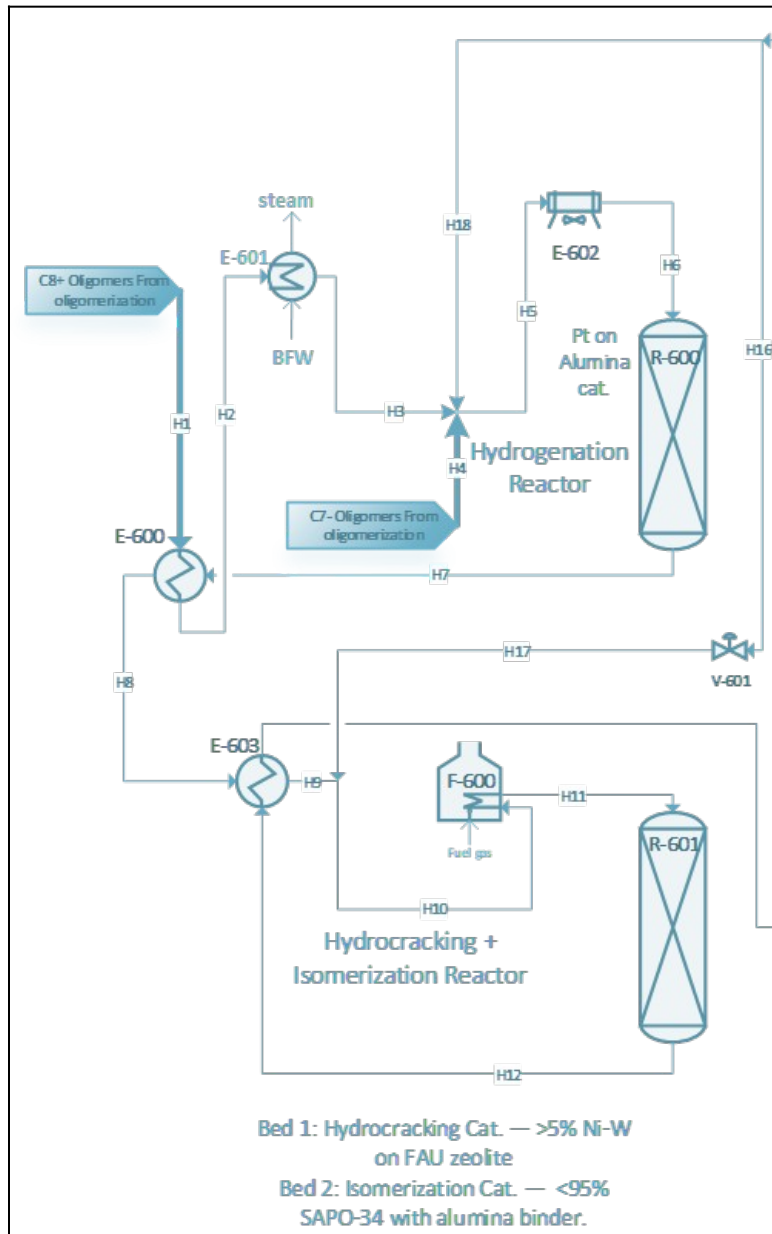
Figure 32- Hydroprocessing Reactions Section
