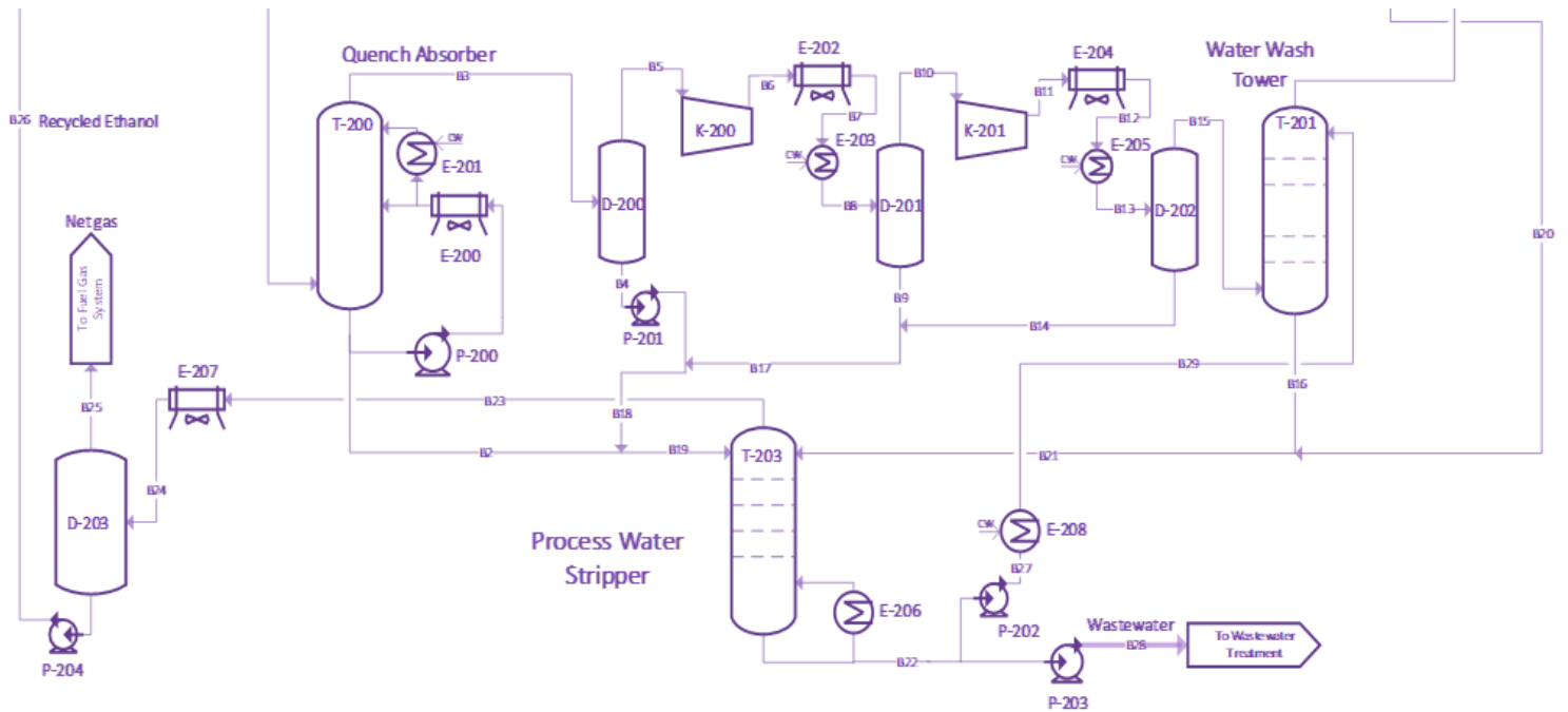
Figure 26- Byproduct Removal Section
