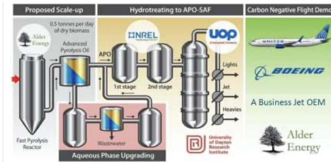
Figure 14: Block flow diagram of Alder Fractionation + UOP hydrotreating
