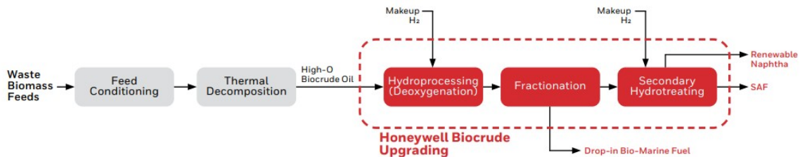
Figure 15- UOP Bio Crude Upgrading BFD
