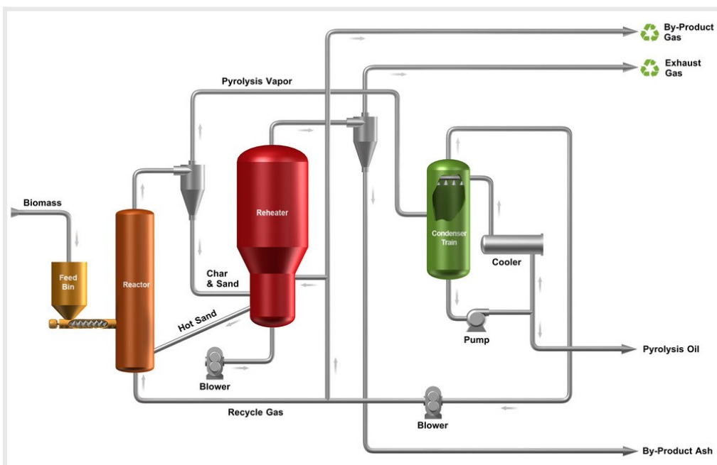
Figure 13:Pyrolysis Block flow diagram
