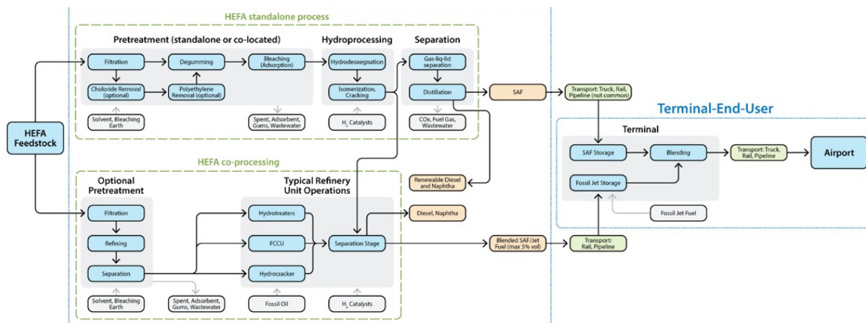
Figure 11: HEFA BFD part 2
