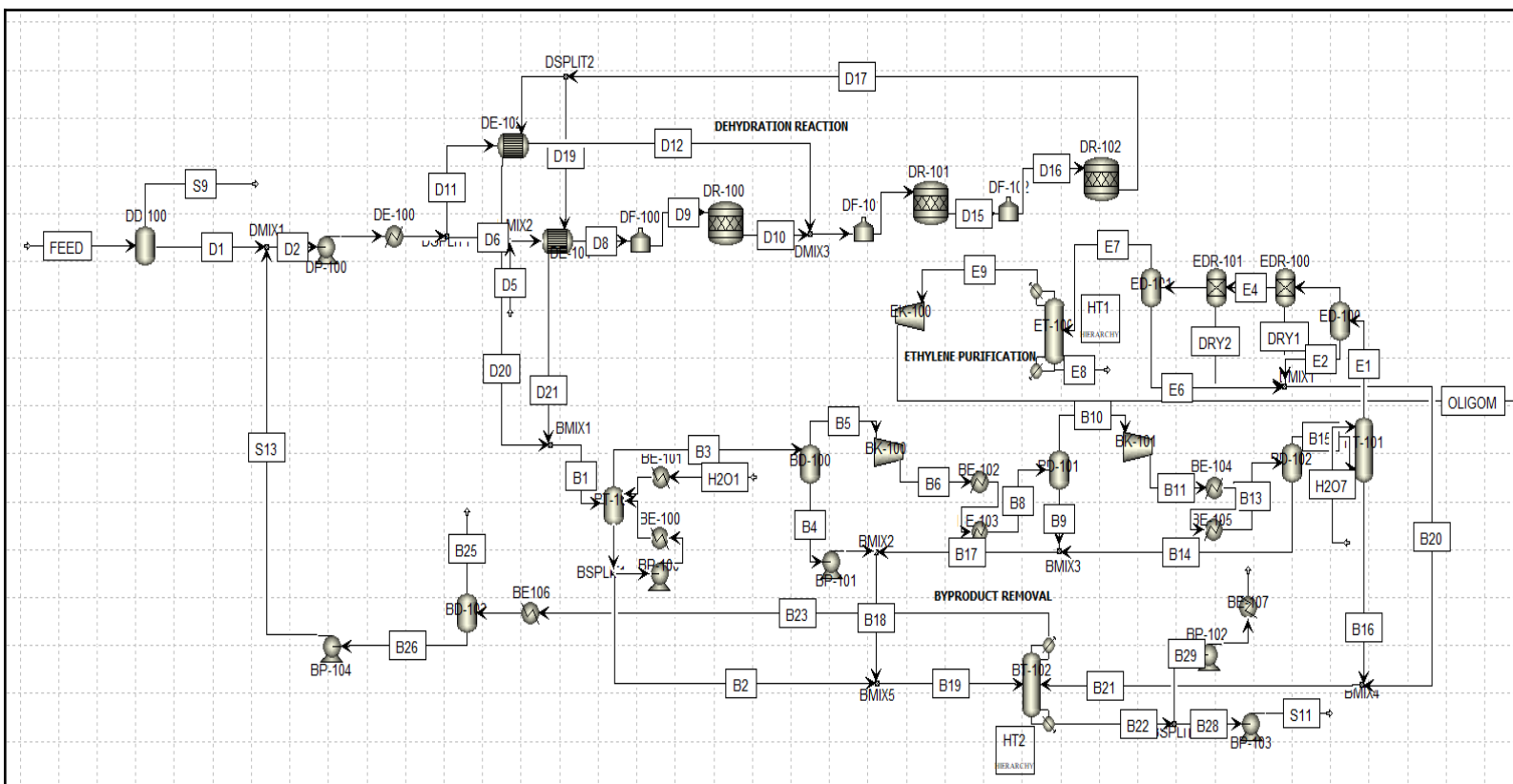
Figure 34- Dehydration of Ethanol to Ethylene Simulation PFD
