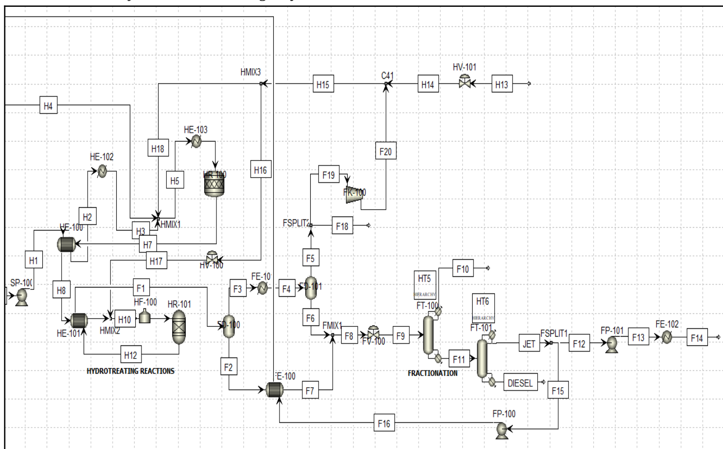
Figure 36- Hydroprocessing of Oligomers to Jet Fuel Simulation PFD
