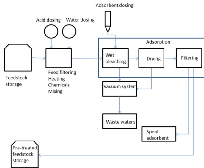
Figure 8: HEFA feedstock pretreatment
