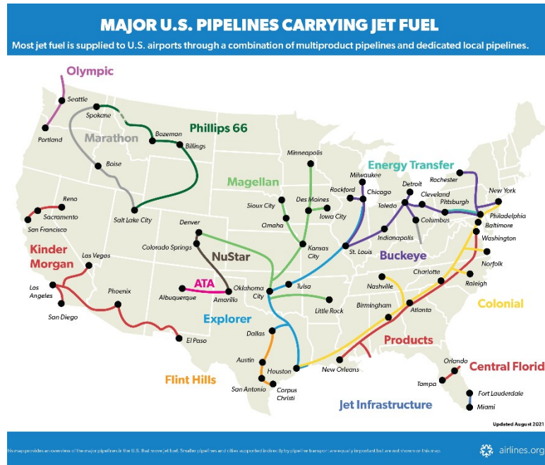
Figure 22 - American Jet Fuel Pipelines
