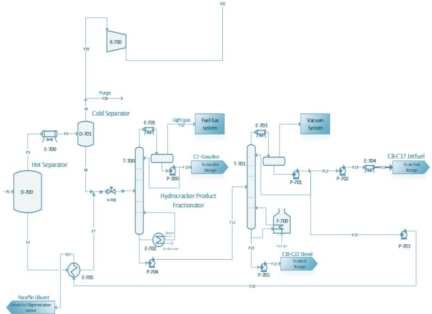
Figure 33- Fractionation of Products Section
